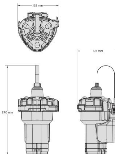
SmartFind G8 EPIRB Range Bracket Assembly
